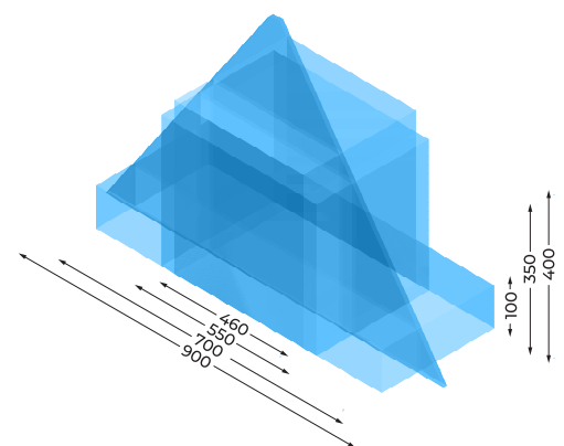
Beam geometry
