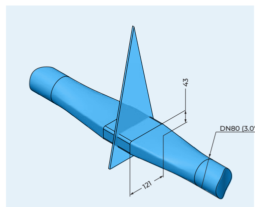
Beam geometry
