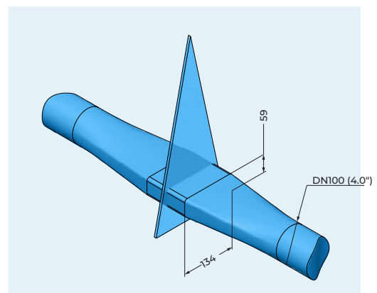
Beam geometry
